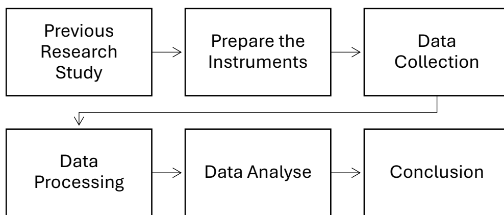
Figure 1. Research Flow
